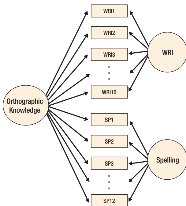
Figure 2 Bifactor Structure of PALS 1–3
